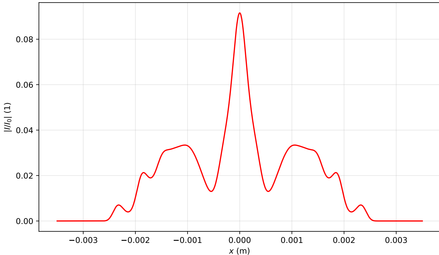
Intensity profile I(x, y = 0, z = 3.582)/I_0 , P_{in}=8.5P_{cr} , artificial time
